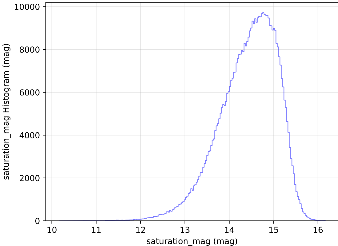
ddf_loaded_half_fl4_v3.4_10yrs All sky i band: saturation_mag Histogram
