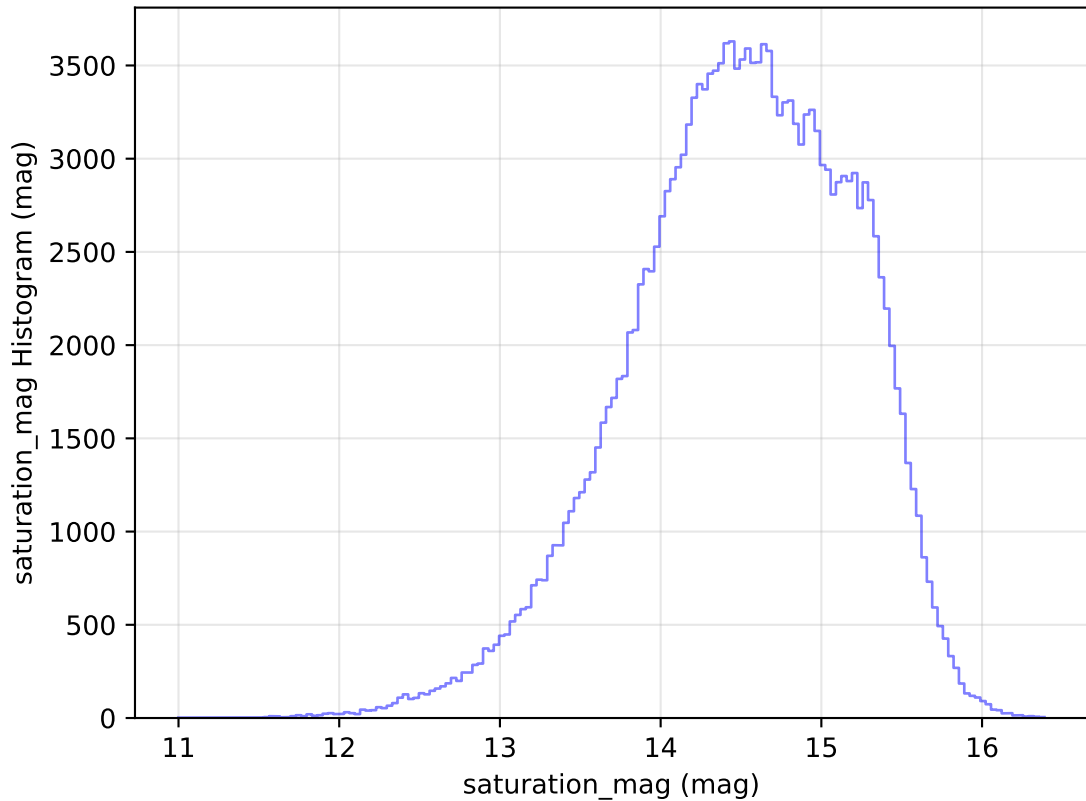
ddf_loaded_half_fl4_v3.4_10yrs All sky g band: saturation_mag Histogram
