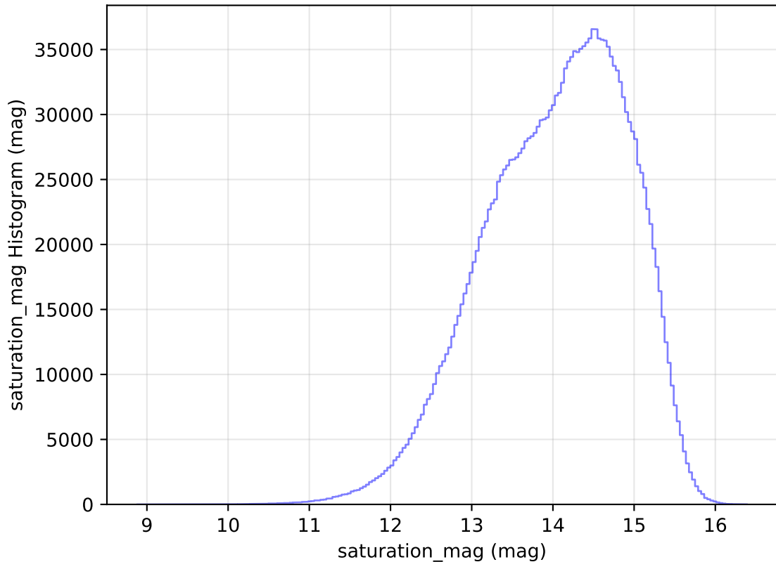
ddf_loaded_half_fl4_v3.4_10yrs All sky all bands: saturation_mag Histogram
