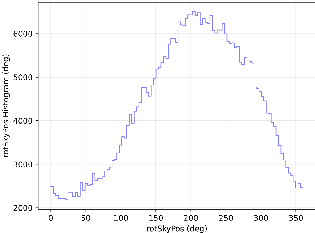
ddf_loaded_half_fl4_v3.4_10yrs WFD z band: rotSkyPos Histogram
