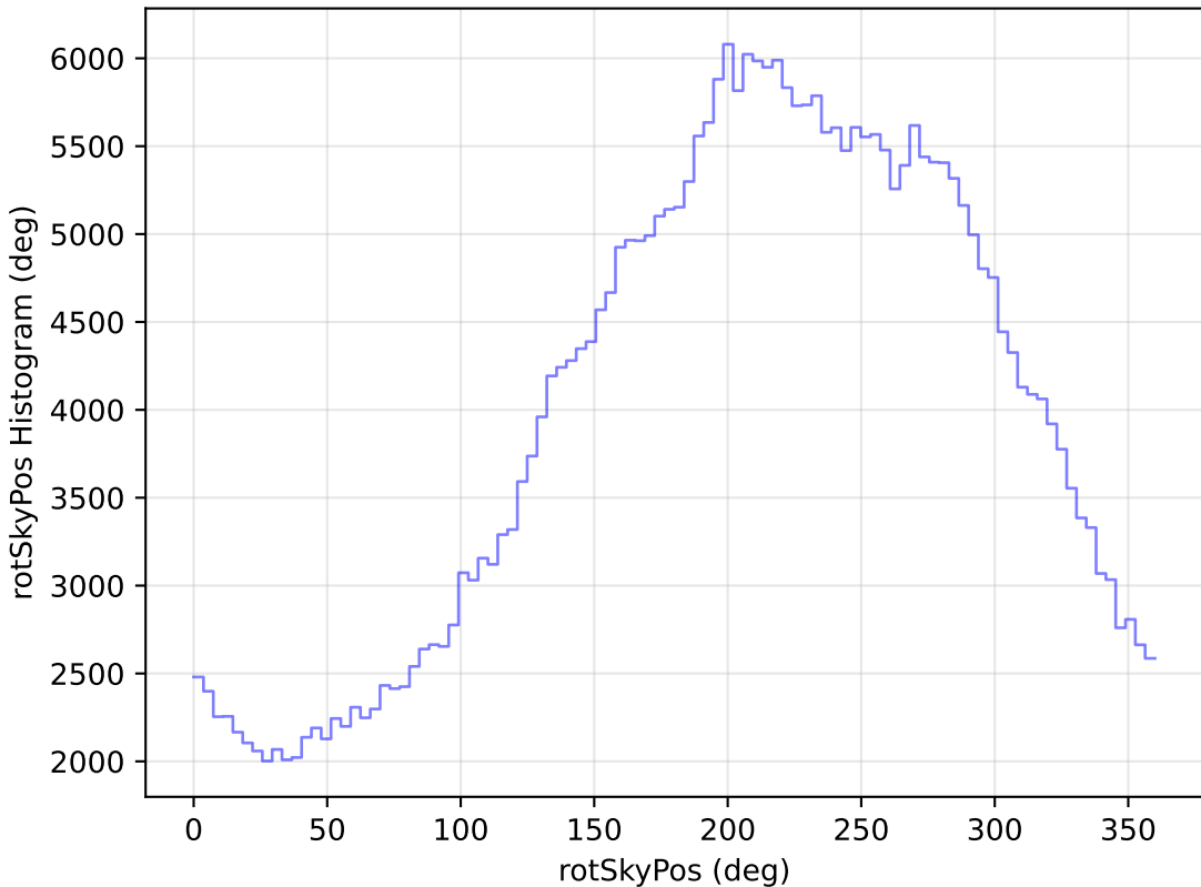
ddf_loaded_half_fl4_v3.4_10yrs WFD y band: rotSkyPos Histogram
