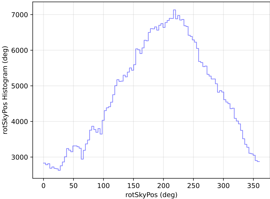
ddf_loaded_half_fl4_v3.4_10yrs WFD r band: rotSkyPos Histogram
