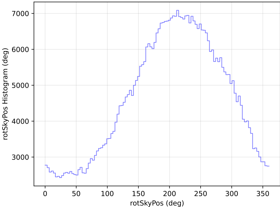
ddf_loaded_half_fl4_v3.4_10yrs WFD i band: rotSkyPos Histogram
