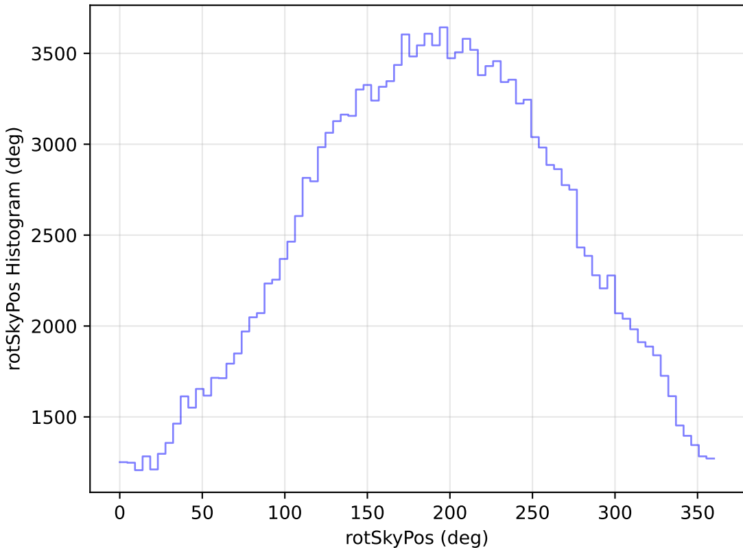
ddf_loaded_half_fl4_v3.4_10yrs WFD g band: rotSkyPos Histogram
