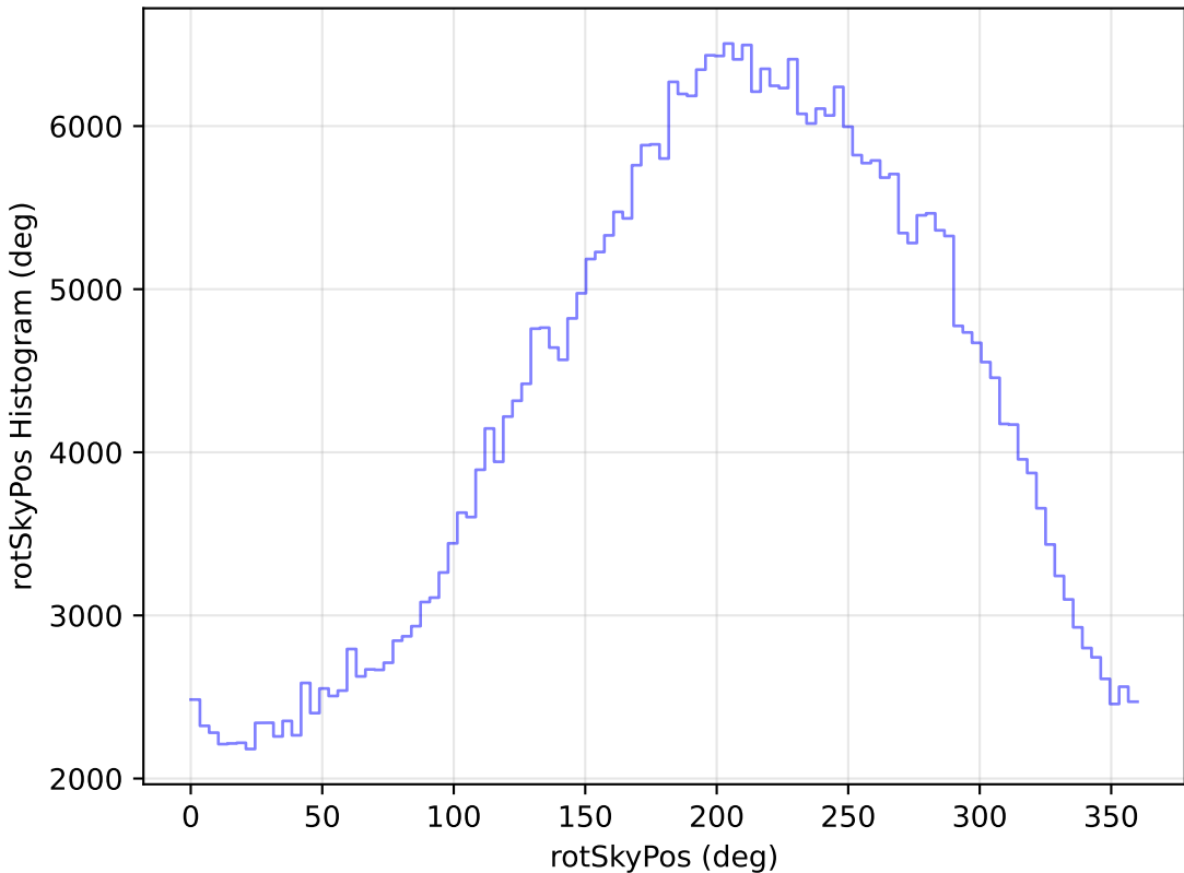
ddf_loaded_half_fl4_v3.4_10yrs All sky z band: rotSkyPos Histogram
