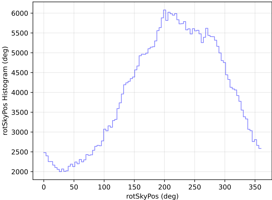
ddf_loaded_half_fl4_v3.4_10yrs All sky y band: rotSkyPos Histogram
