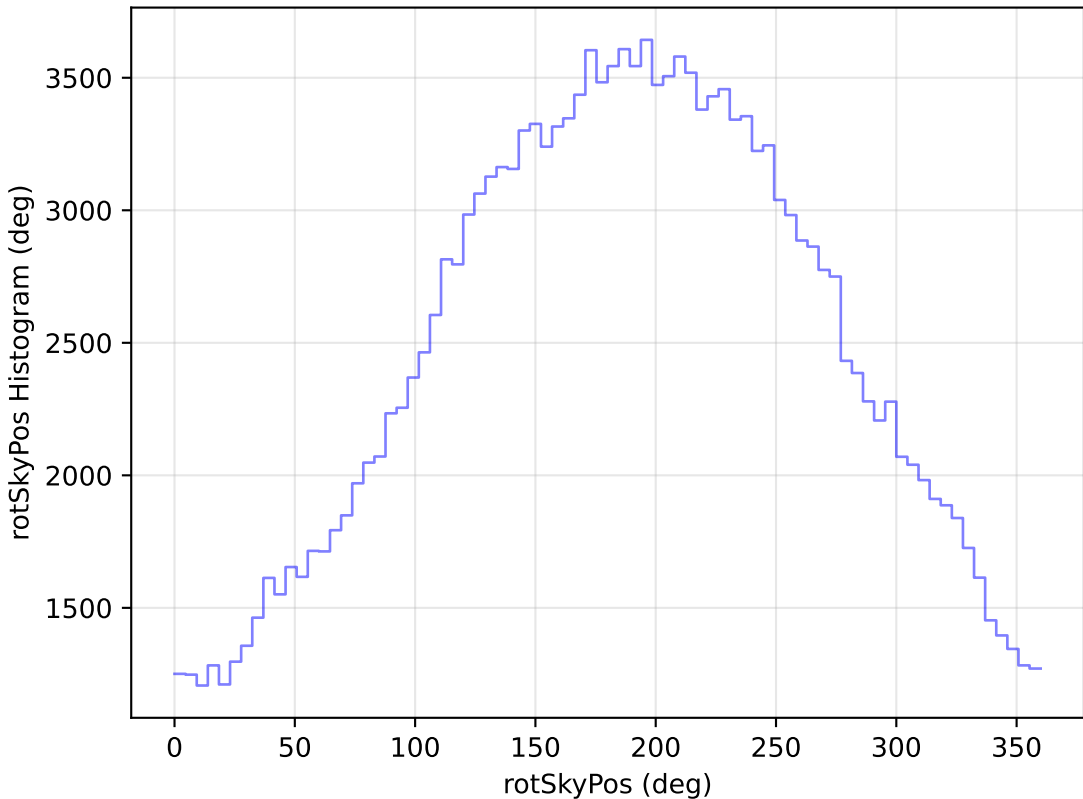
ddf_loaded_half_fl4_v3.4_10yrs All sky g band: rotSkyPos Histogram
