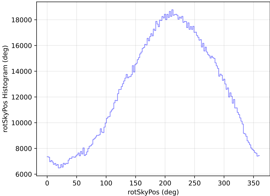
ddf_loaded_half_fl4_v3.4_10yrs All sky all bands: rotSkyPos Histogram
