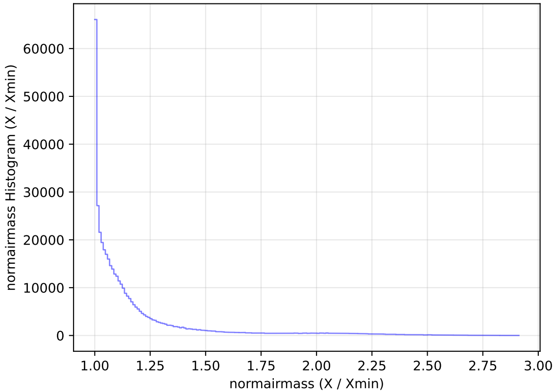
ddf_loaded_half_fl4_v3.4_10yrs WFD z band: normairmass Histogram
