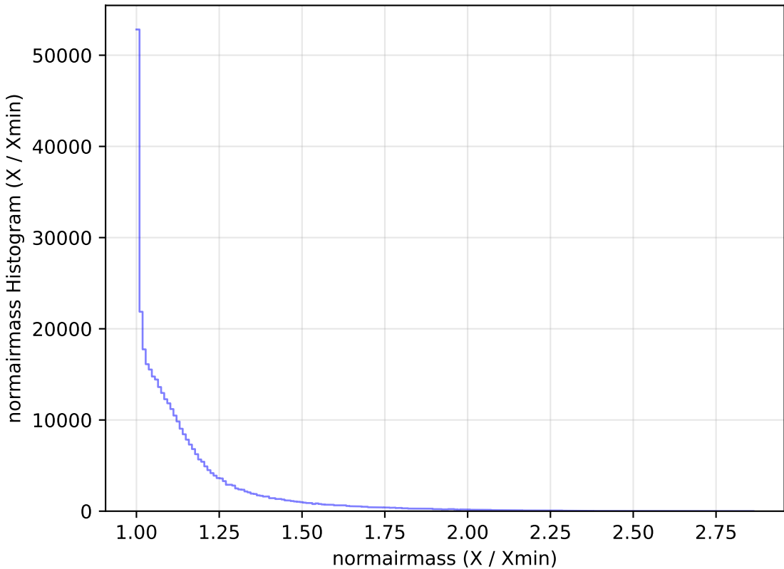
ddf_loaded_half_fl4_v3.4_10yrs WFD y band: normairmass Histogram
