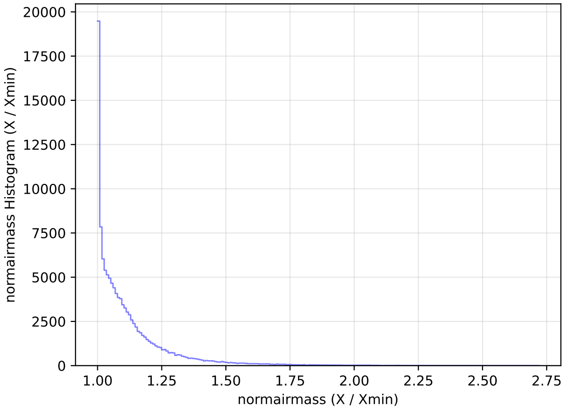
ddf_loaded_half_fl4_v3.4_10yrs WFD u band: normairmass Histogram
