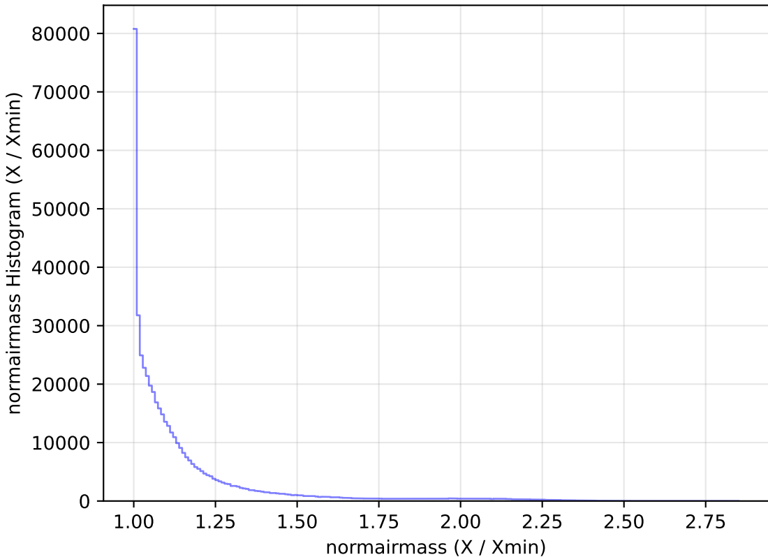
ddf_loaded_half_fl4_v3.4_10yrs WFD r band: normairmass Histogram
