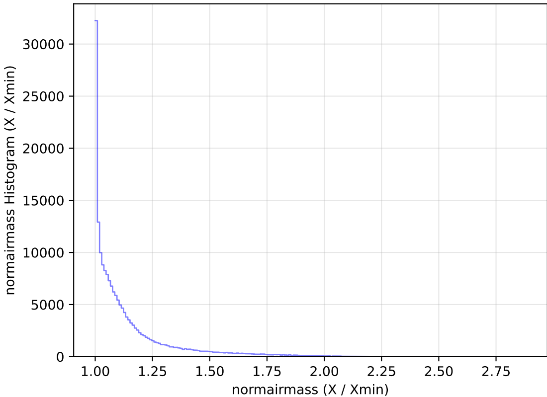
ddf_loaded_half_fl4_v3.4_10yrs WFD g band: normairmass Histogram
