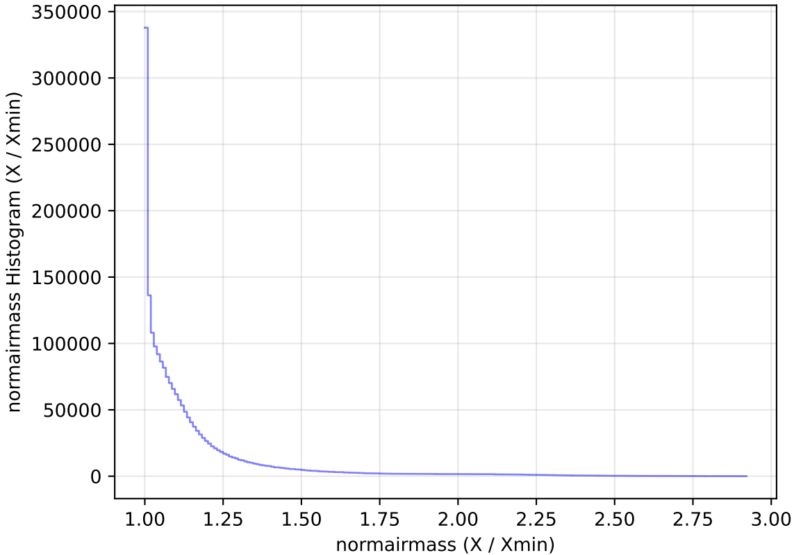
ddf_loaded_half_fl4_v3.4_10yrs WFD all bands: normairmass Histogram
