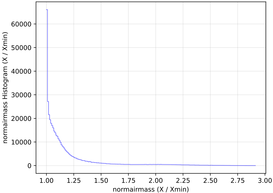
ddf_loaded_half_fl4_v3.4_10yrs All sky z band: normairmass Histogram
