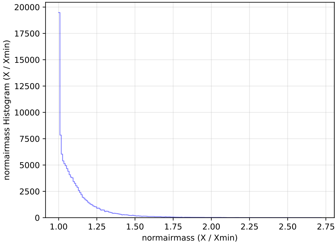
ddf_loaded_half_fl4_v3.4_10yrs All sky u band: normairmass Histogram
