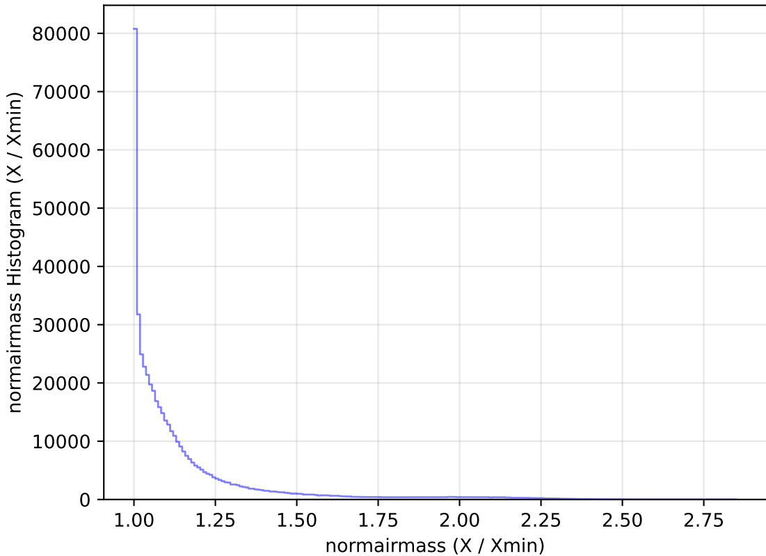
ddf_loaded_half_fl4_v3.4_10yrs All sky r band: normairmass Histogram
