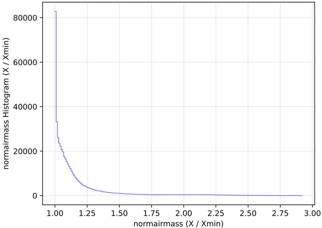
ddf_loaded_half_fl4_v3.4_10yrs All sky i band: normairmass Histogram
