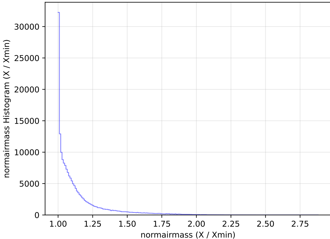
ddf_loaded_half_fl4_v3.4_10yrs All sky g band: normairmass Histogram
