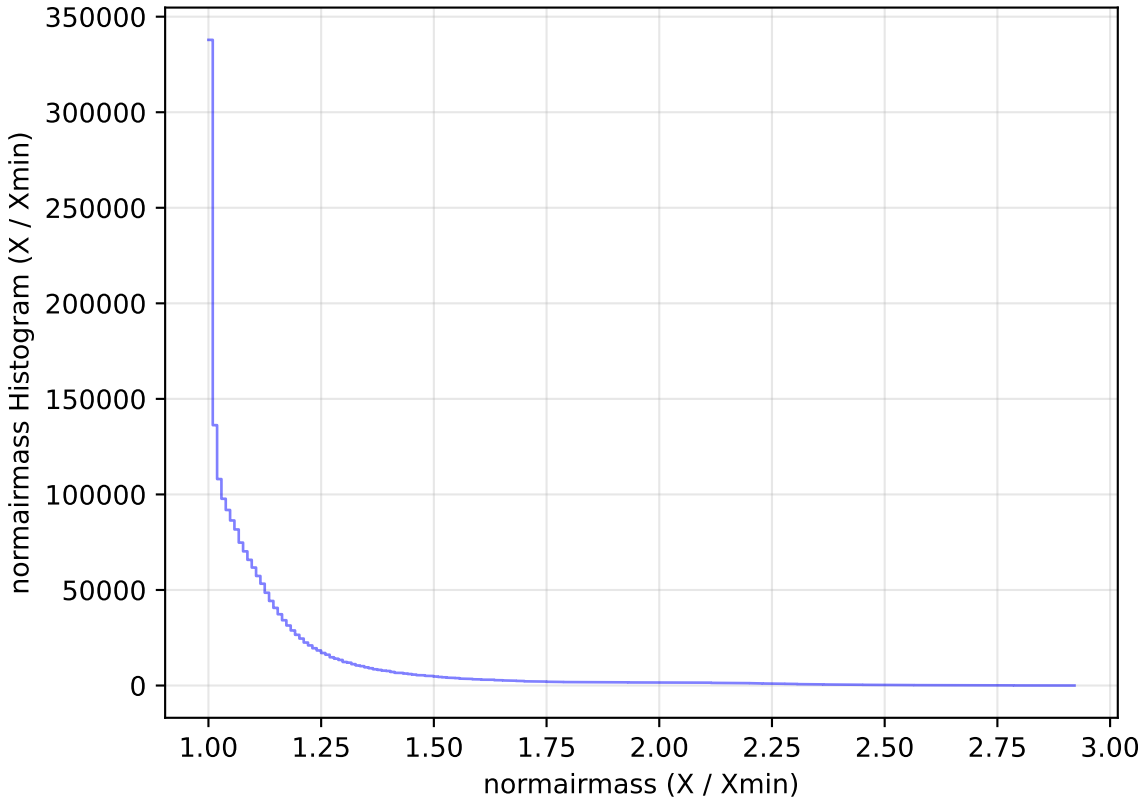
ddf_loaded_half_fl4_v3.4_10yrs All sky all bands: normairmass Histogram
