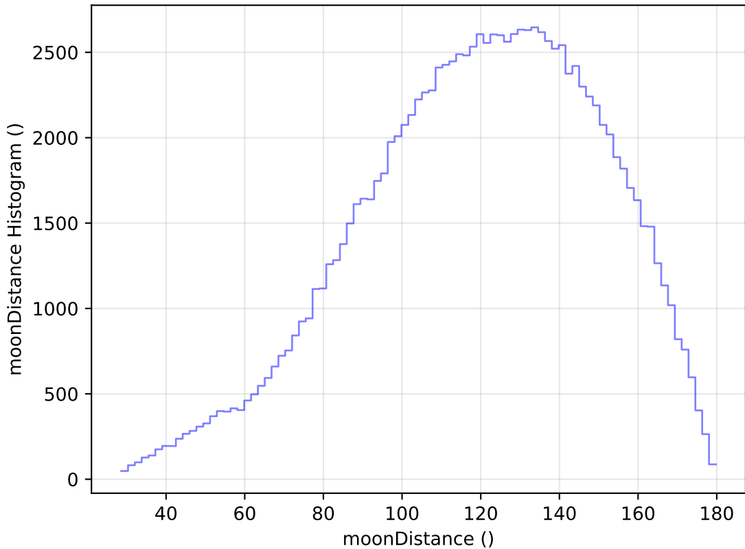
ddf_loaded_half_fl4_v3.4_10yrs WFD u band: moonDistance Histogram
