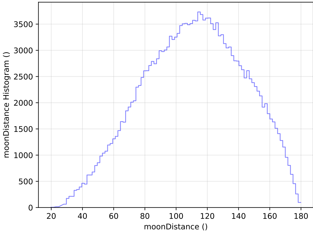
ddf_loaded_half_fl4_v3.4_10yrs WFD g band: moonDistance Histogram
