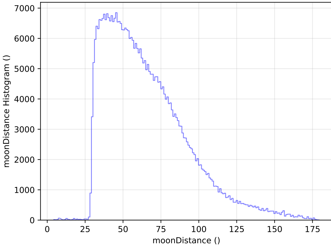
ddf_loaded_half_fl4_v3.4_10yrs All sky y band: moonDistance Histogram
