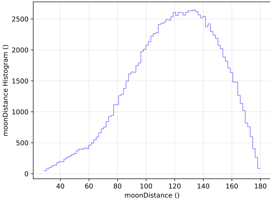
ddf_loaded_half_fl4_v3.4_10yrs All sky u band: moonDistance Histogram
