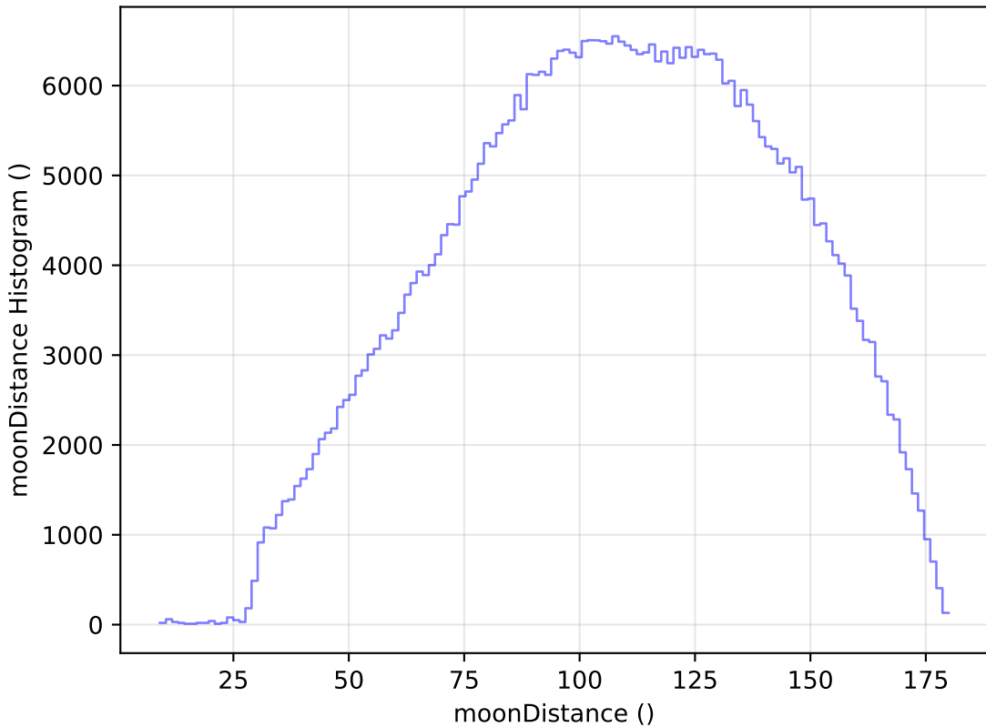
ddf_loaded_half_fl4_v3.4_10yrs All sky r band: moonDistance Histogram
