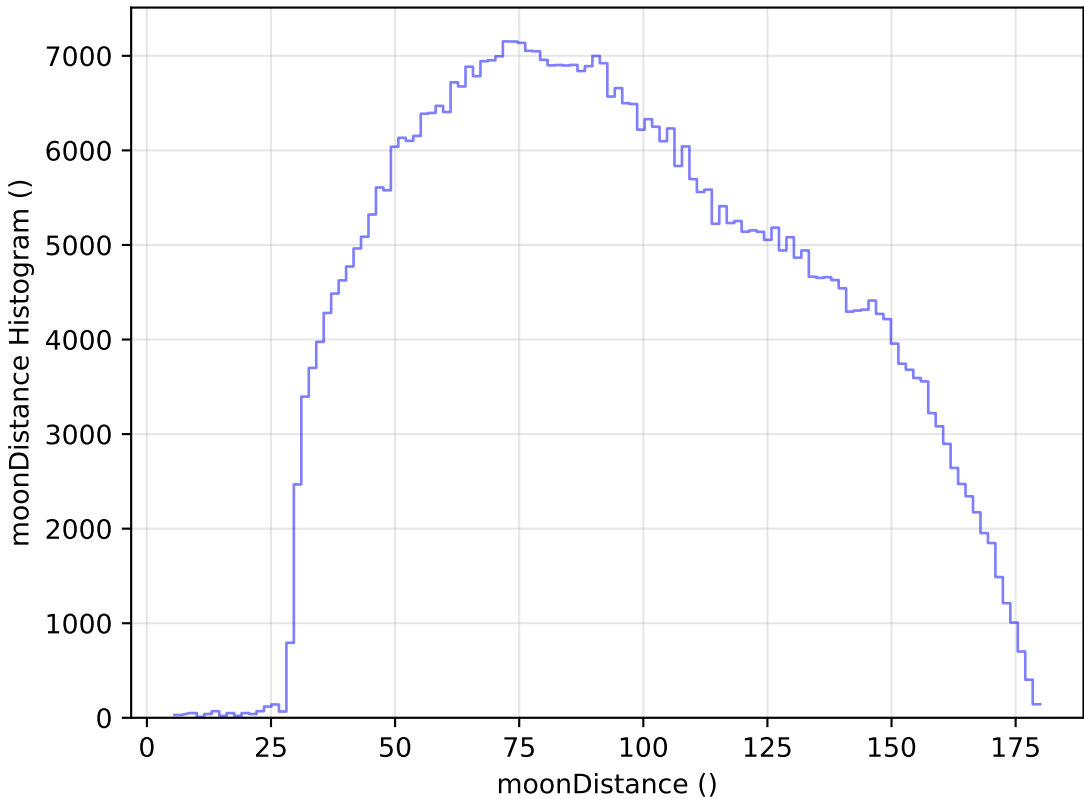
ddf_loaded_half_fl4_v3.4_10yrs All sky i band: moonDistance Histogram
