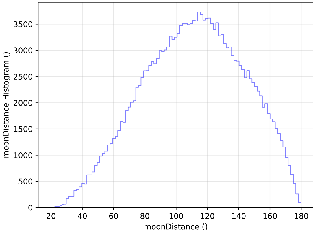
ddf_loaded_half_fl4_v3.4_10yrs All sky g band: moonDistance Histogram
