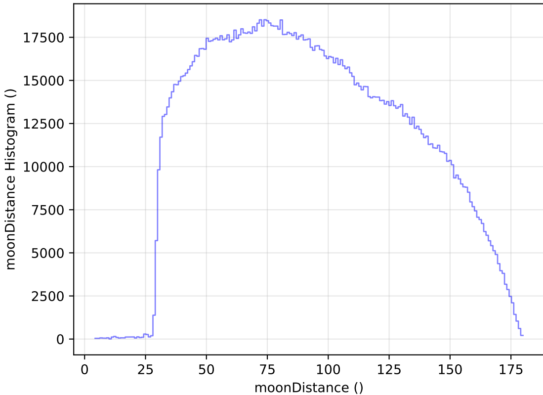
ddf_loaded_half_fl4_v3.4_10yrs All sky all bands: moonDistance Histogram
