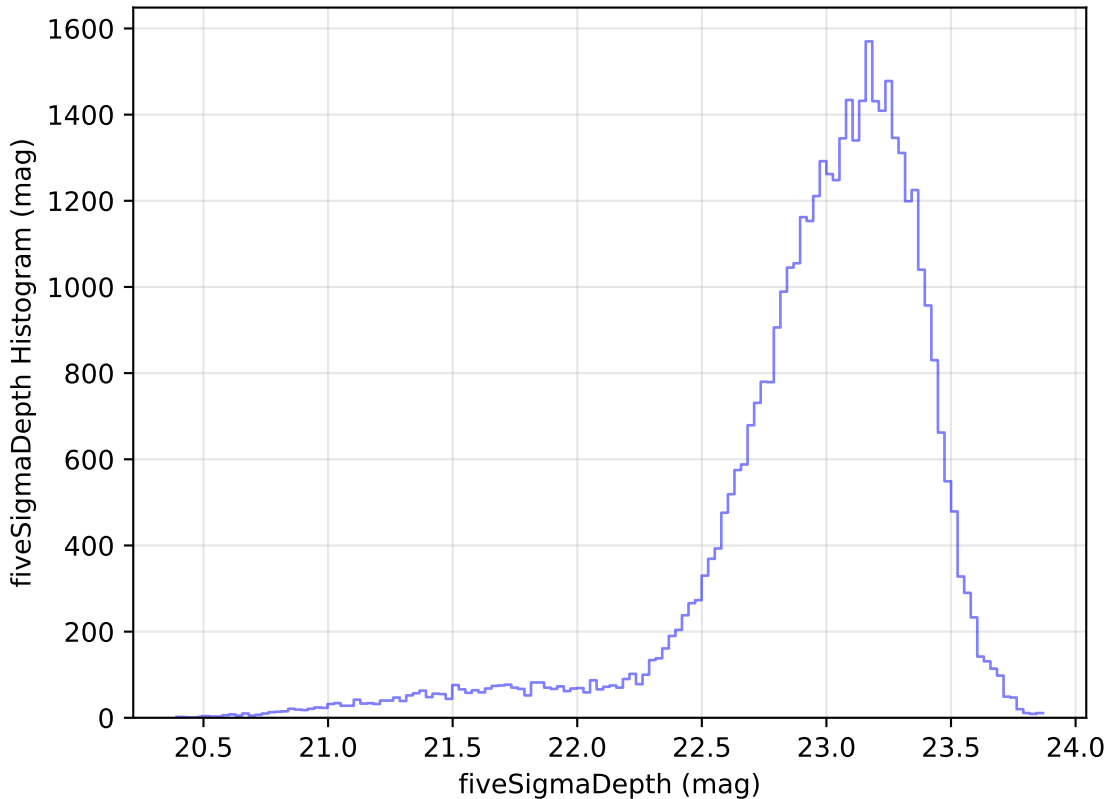
ddf_loaded_half_fl4_v3.4_10yrs Yr 1 z band: fiveSigmaDepth Histogram
