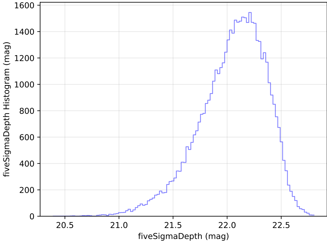
ddf_loaded_half_fl4_v3.4_10yrs Yr 1 y band: fiveSigmaDepth Histogram
