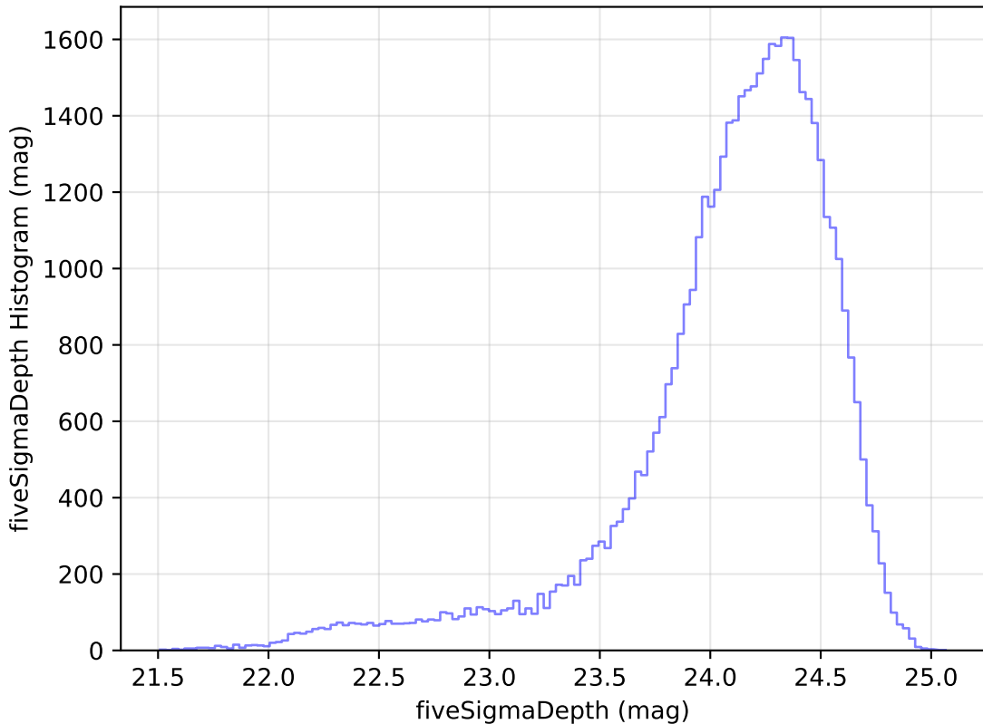
ddf_loaded_half_fl4_v3.4_10yrs Yr 1 r band: fiveSigmaDepth Histogram
