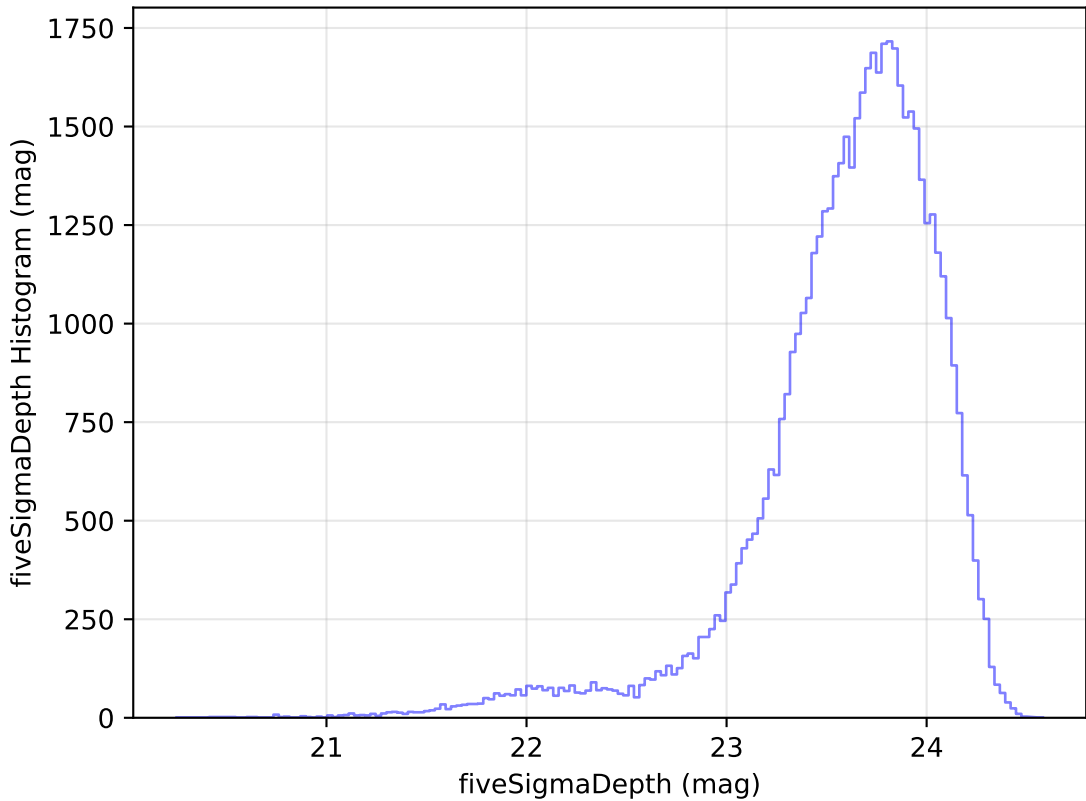
ddf_loaded_half_fl4_v3.4_10yrs Yr 1 i band: fiveSigmaDepth Histogram
