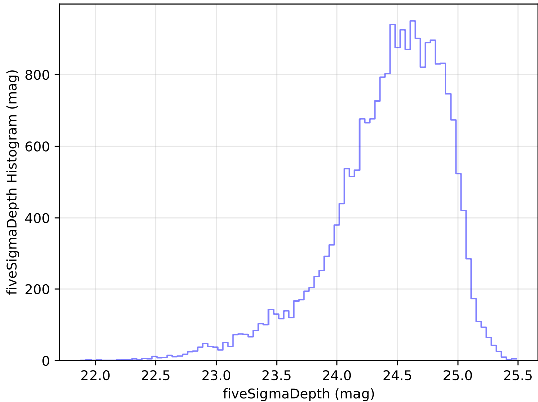
ddf_loaded_half_fl4_v3.4_10yrs Yr 1 g band: fiveSigmaDepth Histogram
