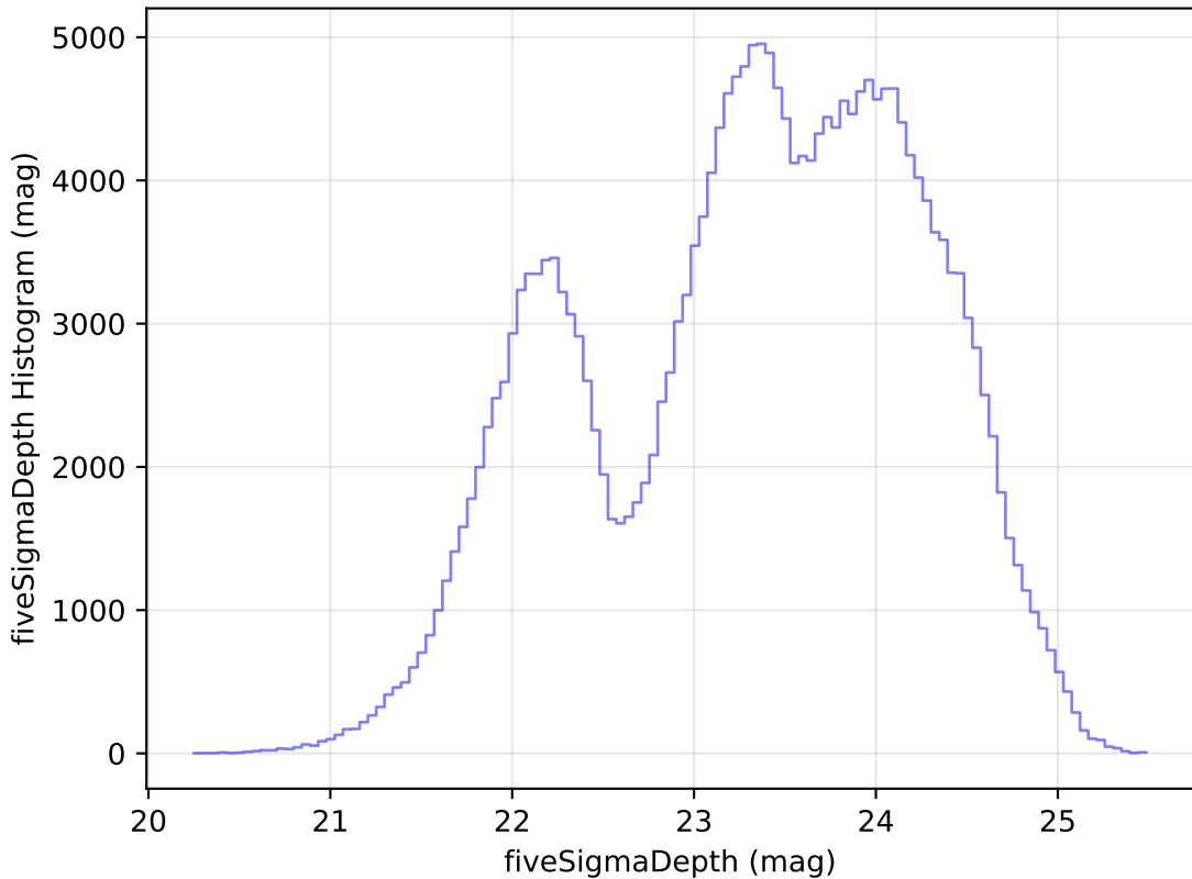
ddf_loaded_half_fl4_v3.4_10yrs Yr 1 all bands: fiveSigmaDepth Histogram
