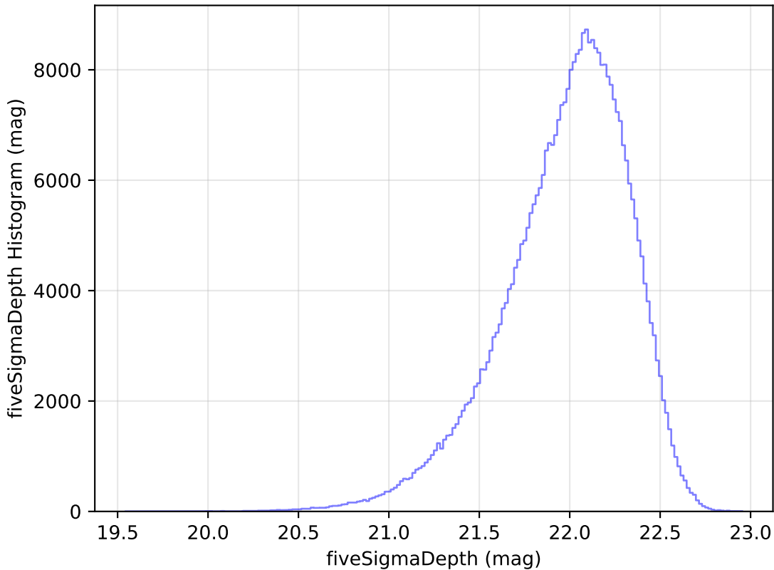
ddf_loaded_half_fl4_v3.4_10yrs WFD y band: fiveSigmaDepth Histogram
