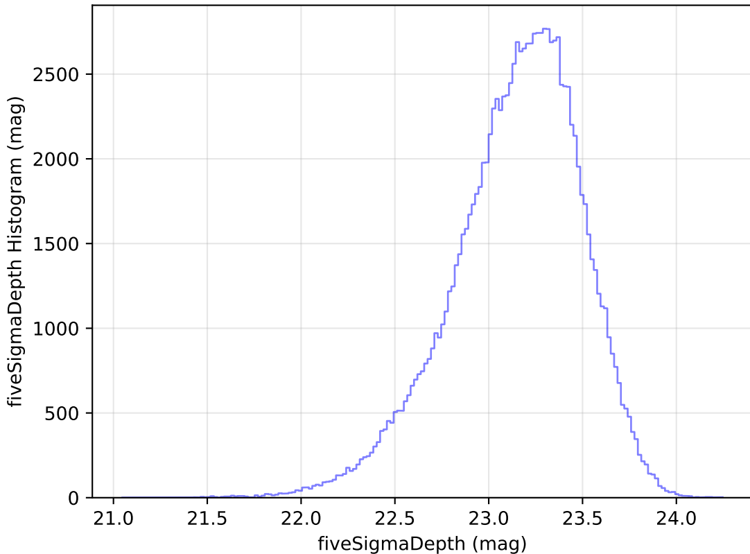
ddf_loaded_half_fl4_v3.4_10yrs WFD u band: fiveSigmaDepth Histogram
