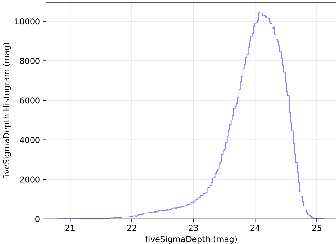
ddf_loaded_half_fl4_v3.4_10yrs WFD r band: fiveSigmaDepth Histogram
