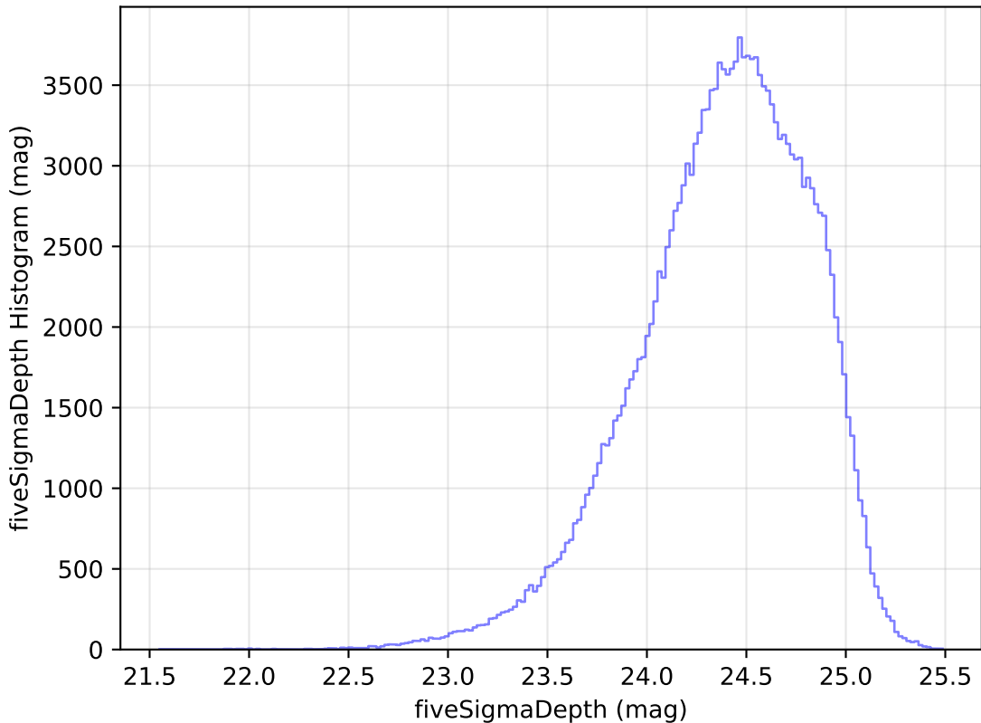
ddf_loaded_half_fl4_v3.4_10yrs WFD g band: fiveSigmaDepth Histogram
