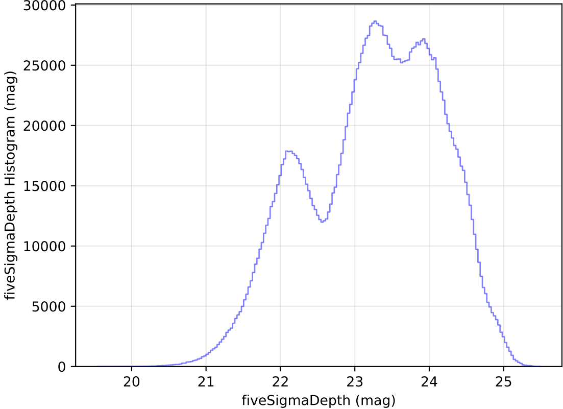
ddf_loaded_half_fl4_v3.4_10yrs WFD all bands: fiveSigmaDepth Histogram
