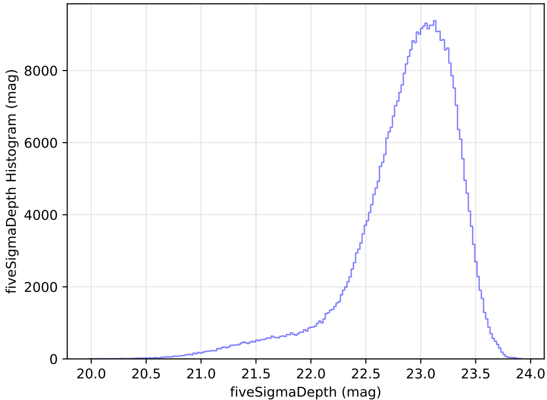
ddf_loaded_half_fl4_v3.4_10yrs All sky z band: fiveSigmaDepth Histogram
