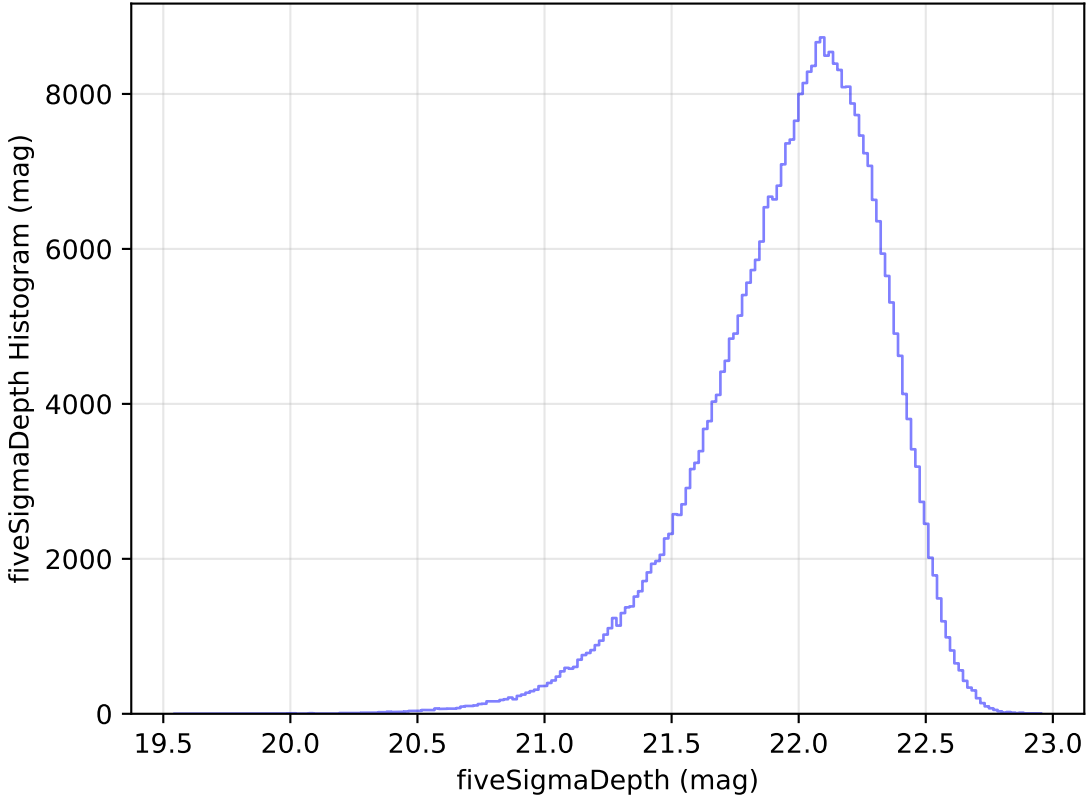
ddf_loaded_half_fl4_v3.4_10yrs All sky y band: fiveSigmaDepth Histogram
