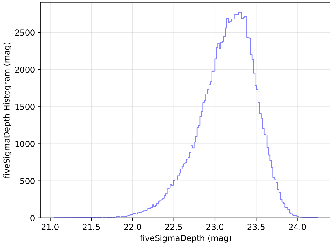
ddf_loaded_half_fl4_v3.4_10yrs All sky u band: fiveSigmaDepth Histogram
