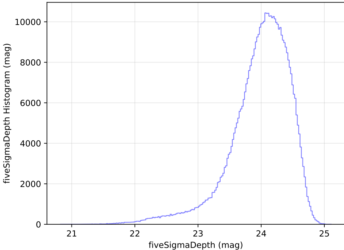
ddf_loaded_half_fl4_v3.4_10yrs All sky r band: fiveSigmaDepth Histogram
