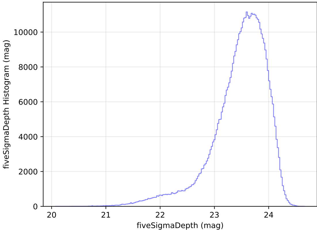
ddf_loaded_half_fl4_v3.4_10yrs All sky i band: fiveSigmaDepth Histogram
