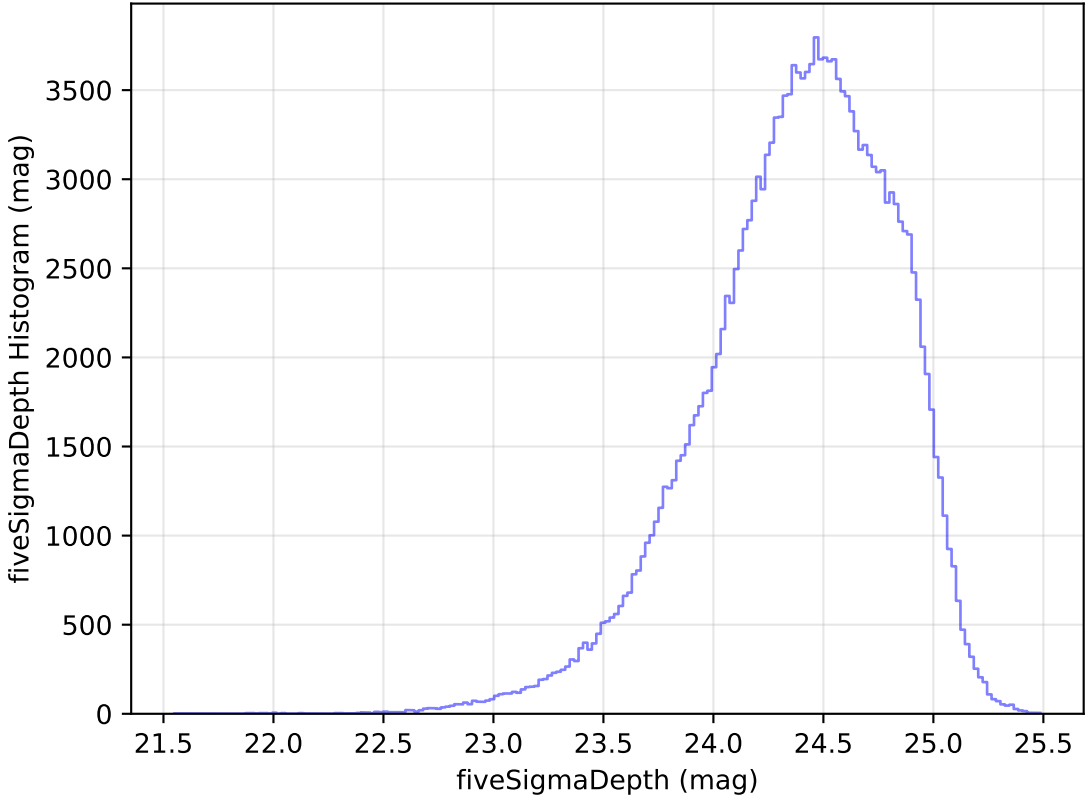
ddf_loaded_half_fl4_v3.4_10yrs All sky g band: fiveSigmaDepth Histogram
