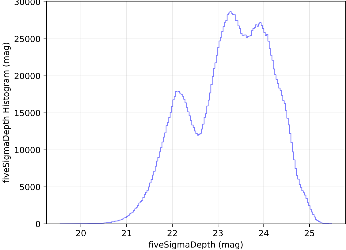
ddf_loaded_half_fl4_v3.4_10yrs All sky all bands: fiveSigmaDepth Histogram
